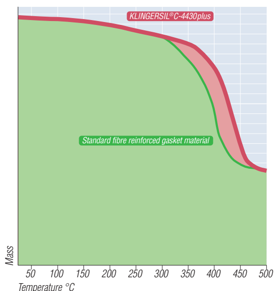
Thermogravimetric analysis
