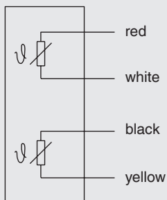
2 x Pt100, 2-wire
