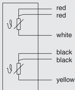
2 x Pt100, 3-wire
